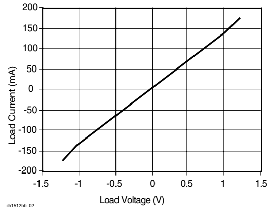
Figure 3. Form A_Typical Load Current vs. Load Voltage
